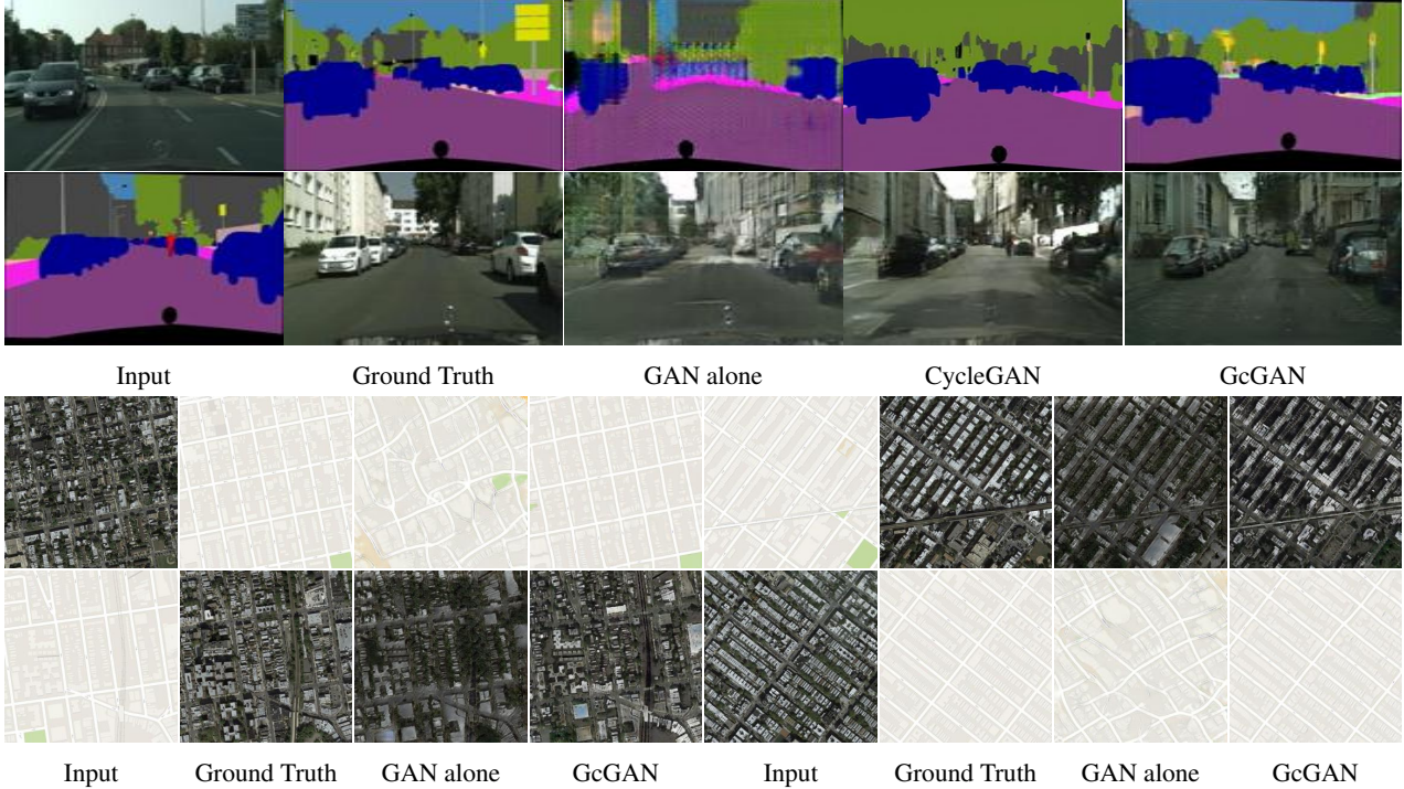
Figure 3: Qualitative comparison on Cityscapes (Parsing \Rightarrow Image) and Google Maps (Map \Rightarrow Aerial photo). GAN alone suffers from mode collapse. Translated images by GcGAN contain more details. GcGAN = GAN\ alone + geometry\ consistency .
