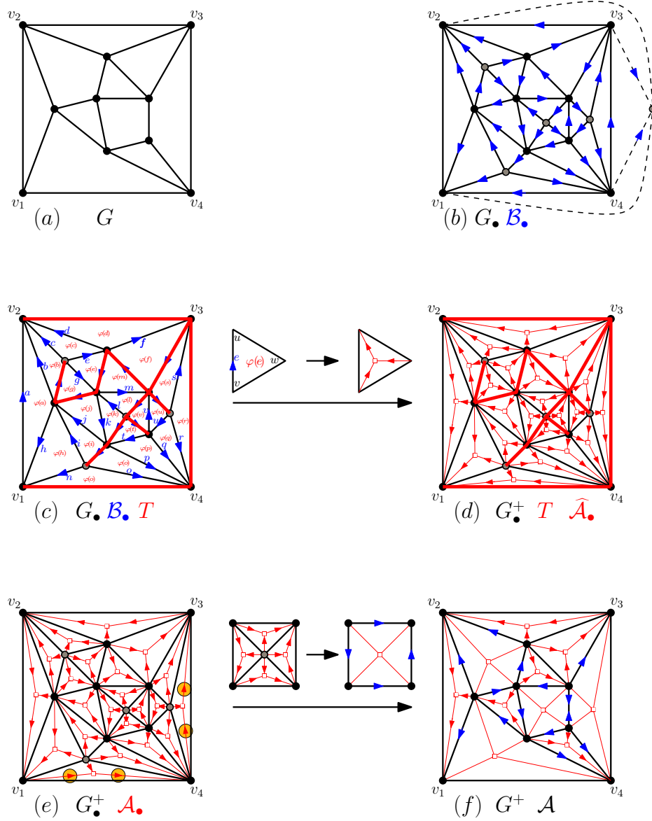
FIGURE 39. Construction of a 4-GS angular orientation \mathcal{A} for a 4-adapted map G . (a) The map G . (b) The triangulation \overline{G}_\bullet with a 3-GS orientation. Restricting the 3-GS orientation to G_\bullet gives an orientation \mathcal{B}_\bullet such every inner-vertex has outdegree 3. (c) A spanning tree T of G_\bullet , oriented from the outer vertices to the inner vertices, and the bijection between the edges in G_\bullet \setminus T and the faces of G_\bullet . (d) Construction of the angular orientation \hat{\mathcal{A}}_\bullet from \mathcal{B}_\bullet . (e) The 4-GS angular orientation \mathcal{A}_\bullet , closely related to \hat{\mathcal{A}}_\bullet (the differences with \hat{\mathcal{A}}_\bullet are highlighted). (f) Construction of the 4-GS angular orientation \mathcal{A} from \mathcal{A}_\bullet .
