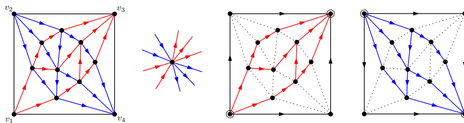
FIGURE 21. From left to right: a transversal structure on a triangulation of the square, the local condition at inner vertices, the red bipolar orientation, and the blue bipolar orientation.
