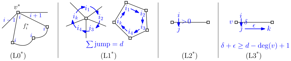
FIGURE 34. Conditions defining dual d -GS labelings.
