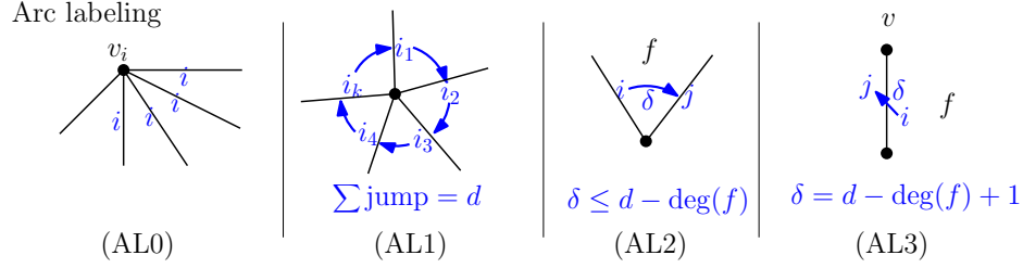
FIGURE 16. The local rules for grand-Schnyder arc labelings.
