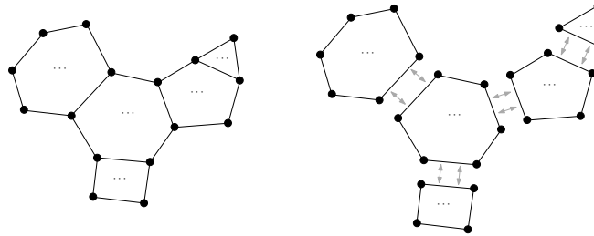
FIGURE 52. Decomposition of a cycle into chordless components.
