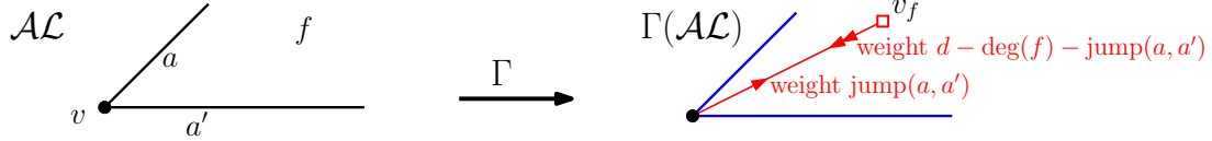
FIGURE 18. Bijection \Gamma = \Psi \circ \Phi \circ \Lambda between the sets \mathbf{AL} of d -GS arc labelings and the set \mathbf{A} of angular orientations for an edge-tight map G
