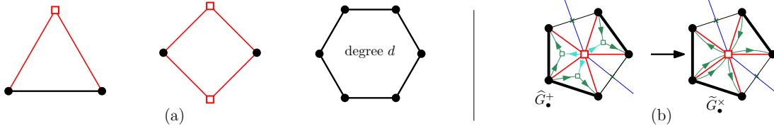
FIGURE 54. (a) The 3 types of inner faces in the map \widehat{G}_\bullet (the second type, arising from special edges of G , does not appear when G is (d+1) -adapted). (b) Contracting the small edges incident to a star vertex of \widehat{G}_\bullet^+ .
