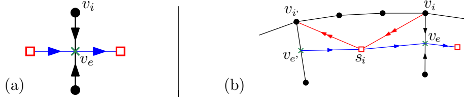
FIGURE 46. (a) A faulty edge e , as defined in the proof of Lemma 12.3. (b) The situation when there exists a faulty edge e .
