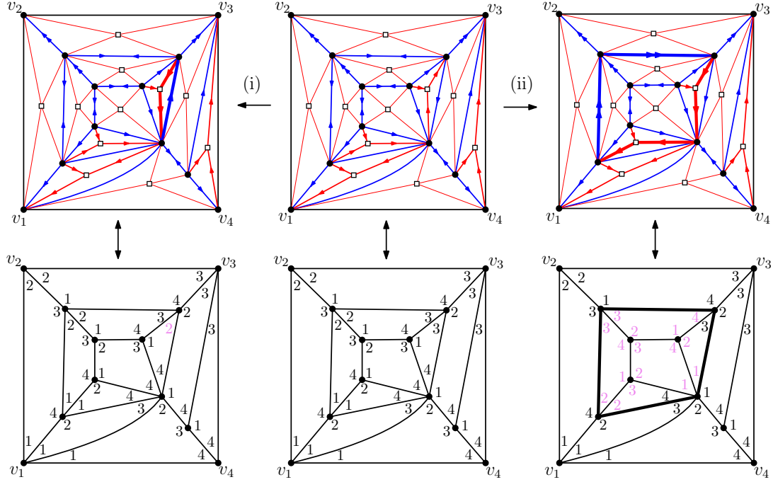
FIGURE 29. The top row shows three 4-GS angular orientations. The left (resp. right) one is obtained from the middle one by pushing an essential clockwise cycle of type (i) (resp. pushing an essential counterclockwise cycle of type (ii)), where the edges of the pushed cycle are shown bolder. The bottom row shows the effect of the push operations on the associated 4-GS labelings, where the modified corner labels are colored.
