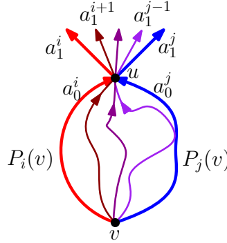
FIGURE 37. The situation in the proof of Lemma 3.9.
