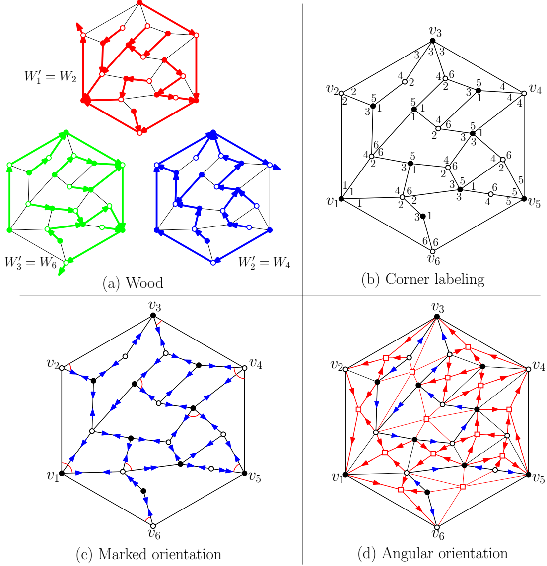
FIGURE 23. Four incarnations of a 3-bipartite-grand-Schnyder structure.
