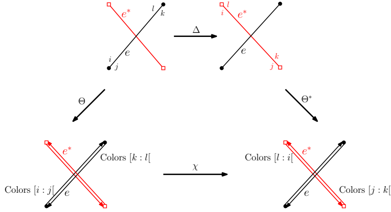
FIGURE 36. The mappings \Theta , \Theta^* and \Delta .
