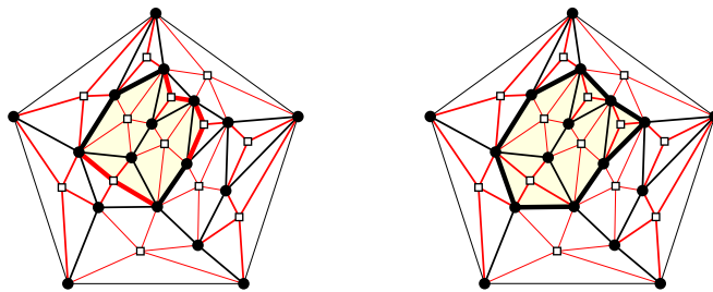
FIGURE 28. Left: a compatible cycle C (shown in bold lines) on the angular map of a 5-map. Right: the same angular map, where the enclosing cycle \hat{C} of C is shown in bold.
