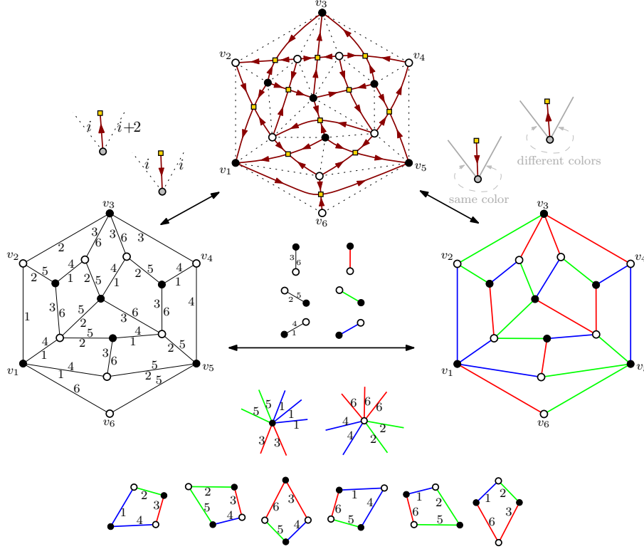
FIGURE 27. On the left, a 3-BGS arc labeling on a quadrangulation of the hexagon. On the right, the corresponding Felsner edge-coloring (upon coloring blue/green/red the outer edges (v_i, v_{i+1}) for i = 1/2/3 modulo 3). The two bottom rows show the local conditions at inner vertices and inner faces (of 6 possible types) when superimposing both structures. The top row shows the associated 3-BGS angular orientation.
