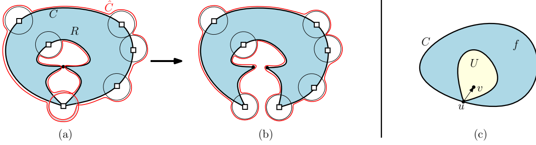
FIGURE 32. (a) A pseudo-compatible C in a map G^+ enclosing a simply connected region R . The star vertices on C are indicated (by squares) together with the contour of the face of G corresponding to these star vertices (represented as circles). For an arc a in \text{Star}(C) , the quantity \ell(a) represents the length of a portion of the contour of the face of G corresponding to the star vertex. Putting together these partial face contours and the arcs in \text{Orig}(C) gives a cycle \hat{C} of G of length \text{enlength}(C) . (b) Duplicating part of the oriented map G^+ , one can get a compatible cycle C' and its enclosing cycle \hat{C}' (in an angular map which is not G^+ ) such that the interior of C' is the same as the interior of C , and the interior of \hat{C}' satisfies the conditions of d -GS orientations (in terms of weights of vertices and edges). (c) Notation for the proof of Theorem 8.1.
