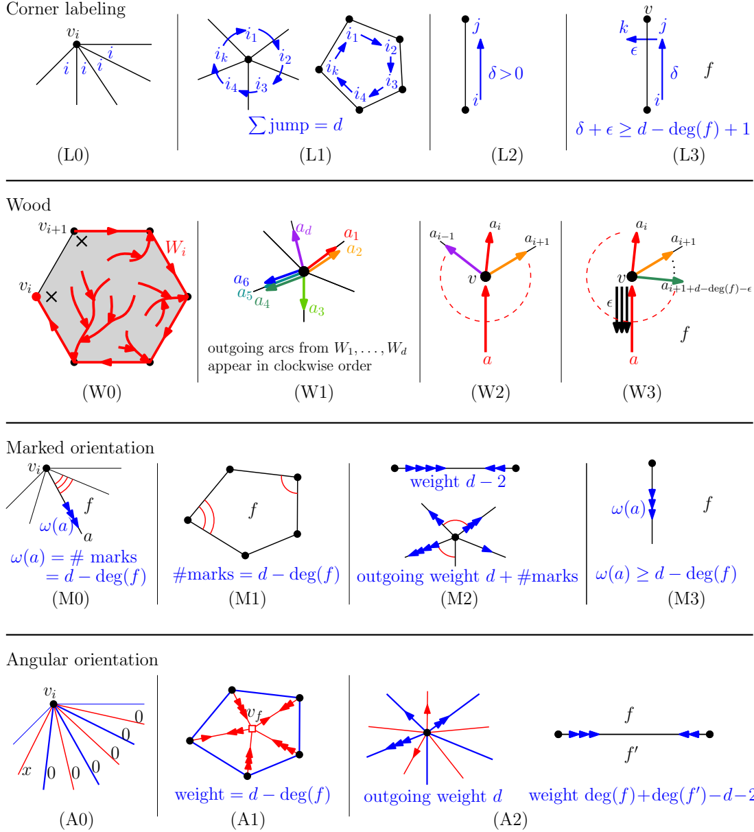
FIGURE 8. Conditions defining the d -grand-Schnyder structures. The orientation weights are indicated by arrowheads (the number of arrowhead indicates the weight), while the markings are indicated by arcs in the corners (the number of arcs indicates the number of marks).
