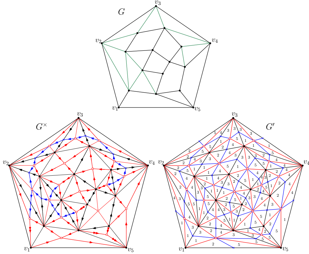
FIGURE 47. Top: a quasi 5-adapted map G (special edges are shown in green). Bottom: on the left a 5-QS angular orientation on G^\times ; on the right the corresponding 5-QS labeling (labeling of the inner faces of G' ).
