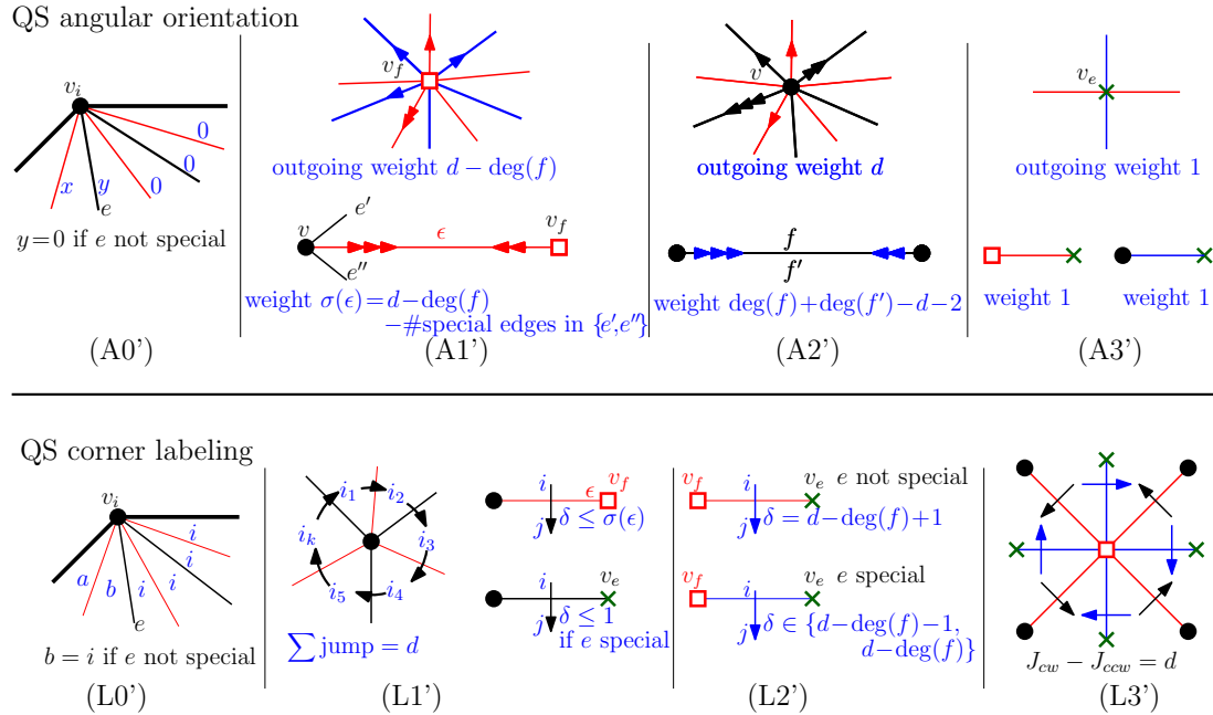
FIGURE 45. Definition of quasi-Schnyder structures.
