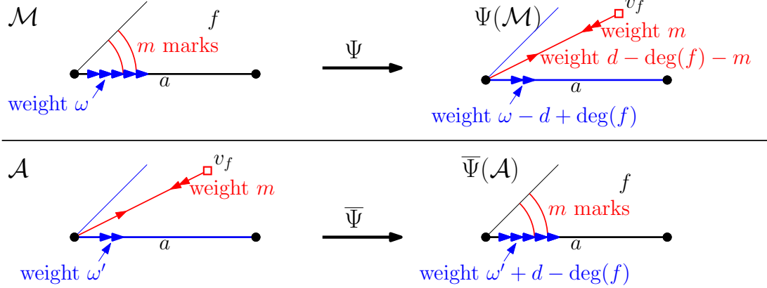
FIGURE 14. Bijection \Psi between d -GS marked orientations and d -GS angular orientations.
