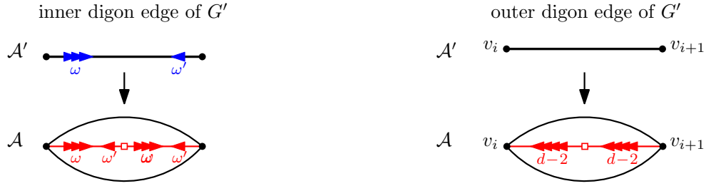
FIGURE 44. The construction of the angular orientation \mathcal{A} starting from \mathcal{A}' . The weights of the arcs in \mathcal{A} and \mathcal{A}' are the same except for digon edges of G' which are transformed as indicated in this figure. The transformation for an inner digon edge is indicated on the left (the weights \omega and \omega' sum to d-2 ), while the transformation of an outer digon edge is indicated on the right. The two edges of G incident to the digon have weight 0.
