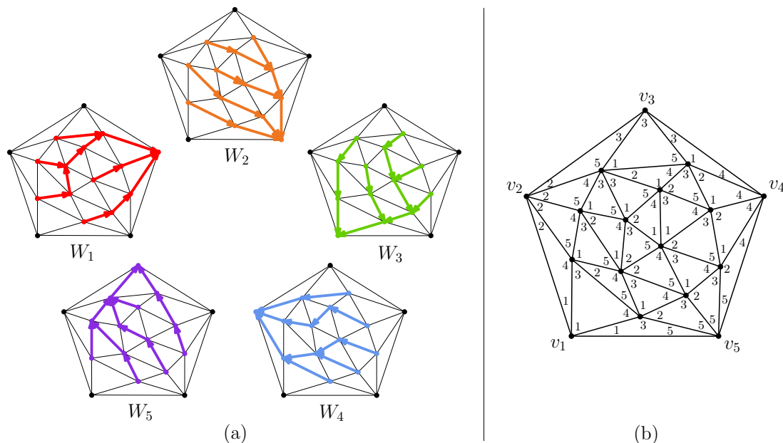
FIGURE 7. (a) A 5-quasi-Schnyder wood of a (quasi 5-adapted) triangulation of a 5-gon. (b) Encoding the quasi-Schnyder structure by a corner labeling.
