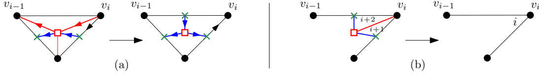
FIGURE 49. Operations to be performed in the neighborhood of outer edges for 5-QS structures of a quasi 5-adapted triangulation. (a) Operations for orientations. (b) Operations for labelings. The configuration shown here is frozen (see Lemma 12.3).
