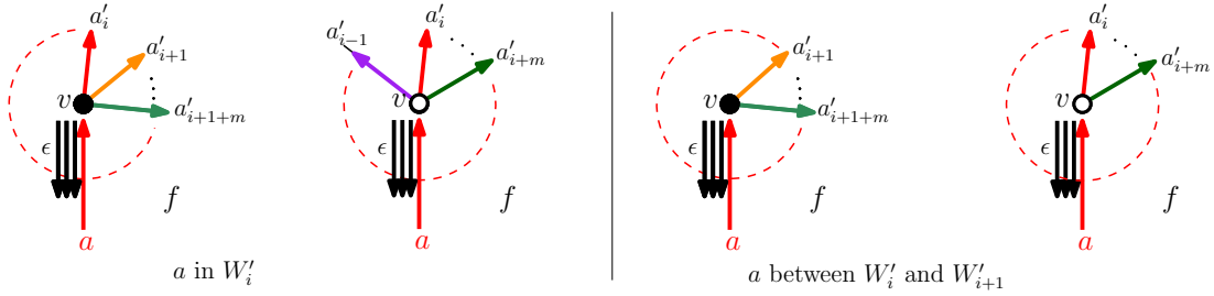
FIGURE 24. Condition (BW2) of b -BGS woods, where m := \max(0, b - \deg(f)/2 - \epsilon) .
