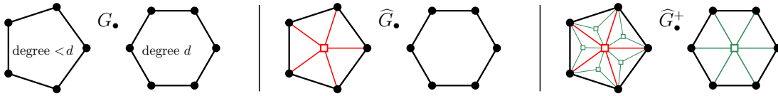
FIGURE 42. The maps G_\bullet , \widehat{G}_\bullet , and \widehat{G}_\bullet^+ . Left: a face of G_\bullet of degree less than d , and a face of degree d . Middle: the corresponding faces in \widehat{G}_\bullet . Right: the corresponding faces in \widehat{G}_\bullet^+ .
