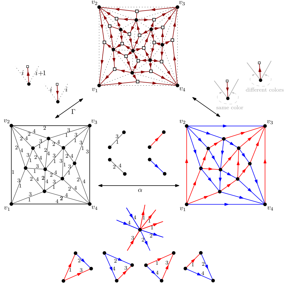
FIGURE 22. On the left, a 4-GS arc labeling on a triangulation of the 4-gon. On the right, the corresponding transversal structure (upon orienting the outer edges from v_1 toward v_3 , and coloring (v_i, v_{i+1}) red/blue for i odd/even). The two bottom rows show the local conditions at inner vertices and inner faces (of 4 possible types) when superimposing both structures. The top row shows the associated 4-GS angular orientation.
