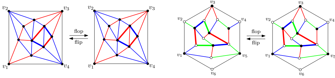
FIGURE 31. Left: a flip/flop operation on a transversal structure, corresponding to an alternating 4-cycle indicated in bold lines. Right: a flip/flop operation on a Felsner edge-coloring, corresponding to an alternating 6-cycle indicated in bold lines.
