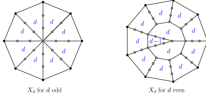
FIGURE 41. The (d+1) -map X_d in the case of odd d (left, represented for d = 7 ) and in the case of even d (right, represented for d = 8 ). The degree of the inner faces are indicated (the outer face has degree d+1 ).
