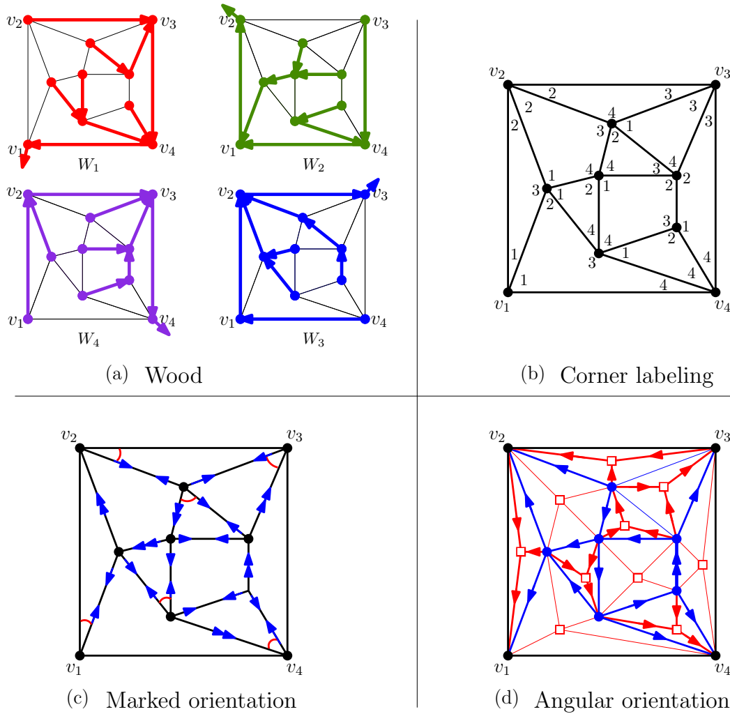
FIGURE 4. Four incarnations of the same 4-grand-Schneider structure.
