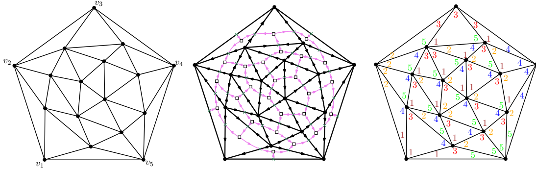
FIGURE 50. Left: A quasi 5-adapted triangulated map G . Middle: the primal-dual completion of G , endowed with a 5-QS angular orientations (more precisely, the orientation obtained from 5-QS angular orientations by applying the operations of Figure 49(a), and deleting the star edges). Right: the corresponding 5-QS labeling of G (more precisely, the corner labeling of G obtained from the 5-QS labeling by applying the operations of Figure 49(b), and transferring the labels from inner faces of G' to inner corners of G ).
