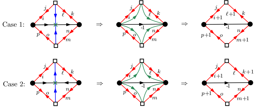
FIGURE 51. Starting from a d -QS angular orientation, and applying the shown local rules at every edge-vertex, one obtains a relaxed d -GS angular orientation (arcs with no weight indication have weight 1, arcs not shown on their edge have weight 0).
