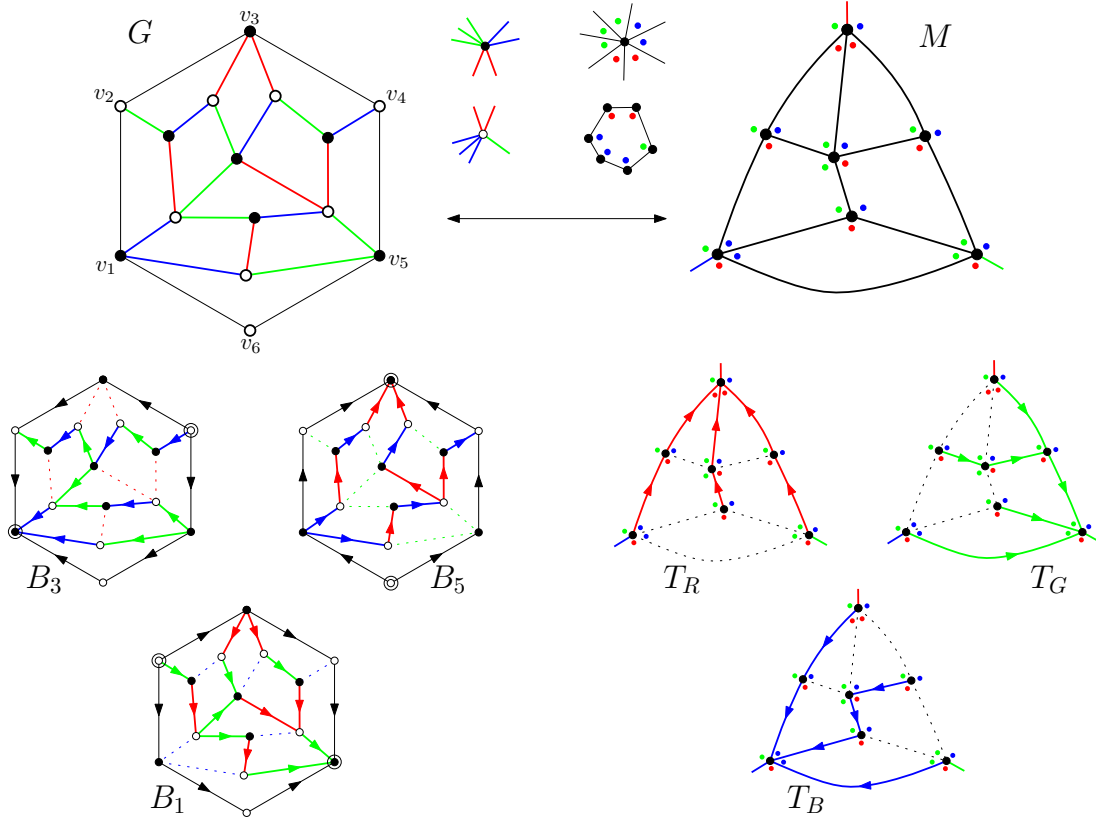
FIGURE 26. On the left, a Felsner edge-coloring of an quadrangulation of the hexagon, and the 3 associated bipolar orientations (blue-green, red-blue, and green-red). On the right, the corresponding coloring of corners of the diagonal-map, and the 3 associated spanning trees.
