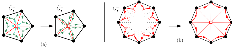
FIGURE 43. (a) Contracting the small edges incident to a star vertex of G_\bullet^+ . (b) Getting from the orientation \mathcal{A}_\bullet of G_\bullet^+ to the orientation \mathcal{A} of G^+ (situation inside a copy of X_d ).
