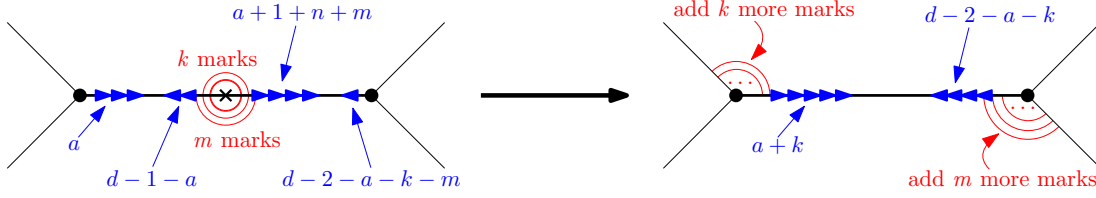
FIGURE 25. Merge an edge of \bar{G} .
