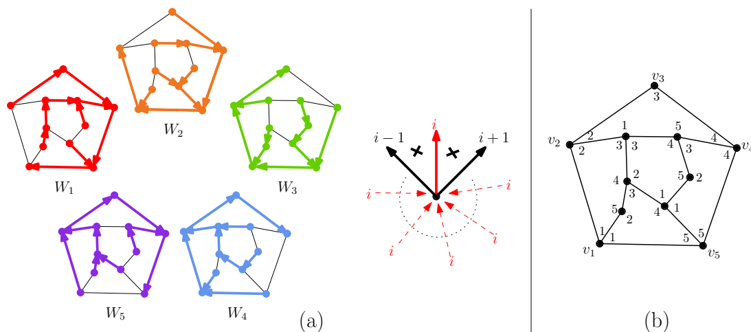
FIGURE 3. (a) The five trees forming the 5-Schnyder decomposition. (b) Encoding the Schnyder decomposition by a corner labeling.
