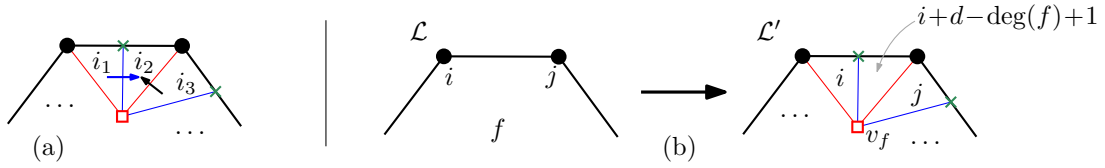
FIGURE 48. (a) Situation described in Remark 12.6 (the inequality \text{jump}(i_1, i_2) \geq \text{jump}(i_3, i_2) always holds). (b) Turning a d -GS labeling into a d -QS labeling.
