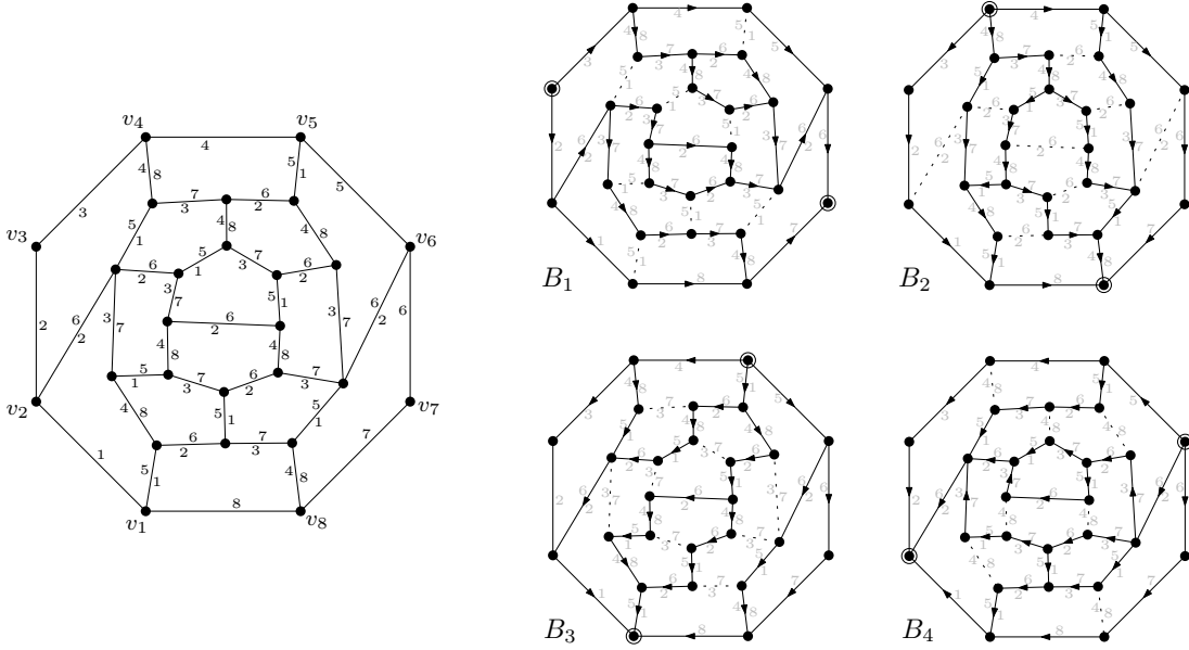
FIGURE 20. Left: an edge-tight pentagulated 8-adapted map endowed with an 8-GS arc labeling. Right: the 4 associated plane bipolar orientations B_1, B_2, B_3, B_4 .
