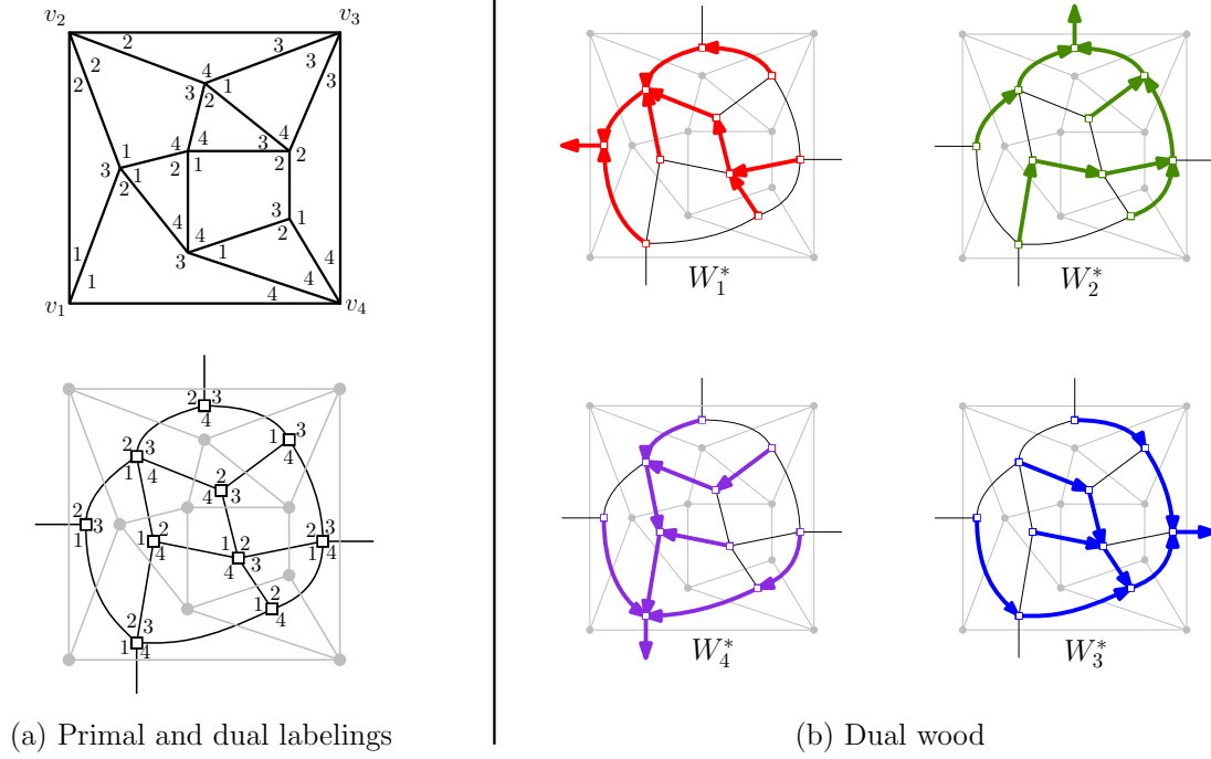
FIGURE 33. Wood and labeling of a dual 4-GS structure.
