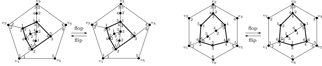
FIGURE 30. Left: a flip/flop operation on a 5-GS corner labeling of a pentagulation. Right: a flip/flop operation on a 3-BGS corner labeling of a hexangulation.
